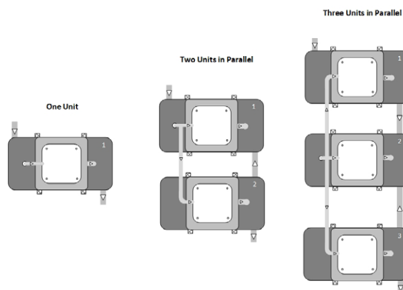
Top view schematic drawing of the Tower Plus - one stage configurations
