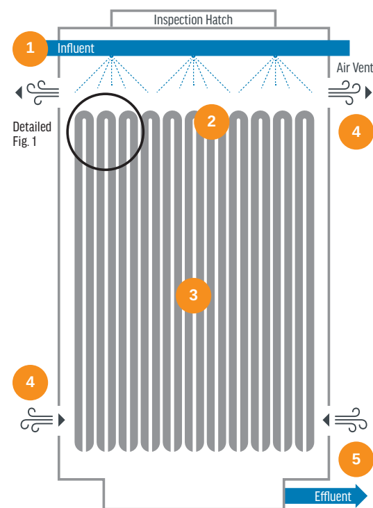
Fig. 2. BioGill Tower Process Flow
