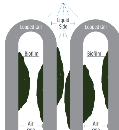
Fig. 1. Gill Structure
